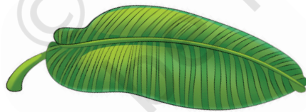
(b) Banana leaf with parallel venation
