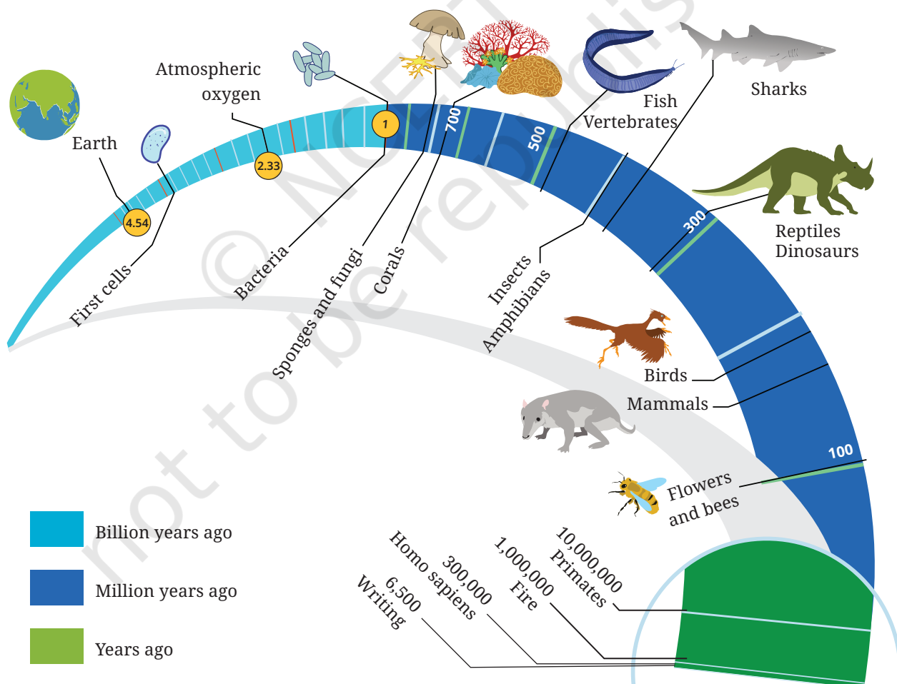
Fig. 4.1. Timeline of a few important stages in the evolution of life on Earth.
