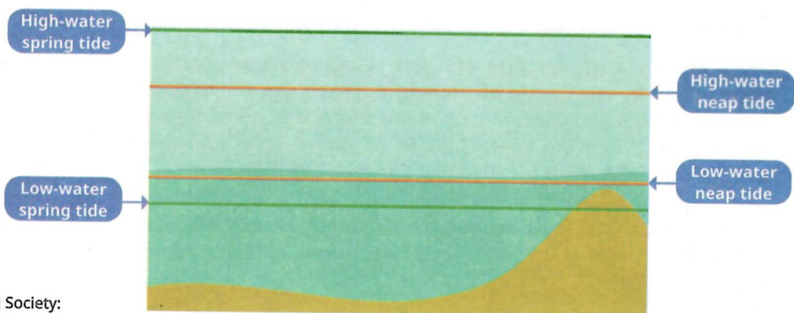
Fig. 1.6. Levels of spring and neap tides
