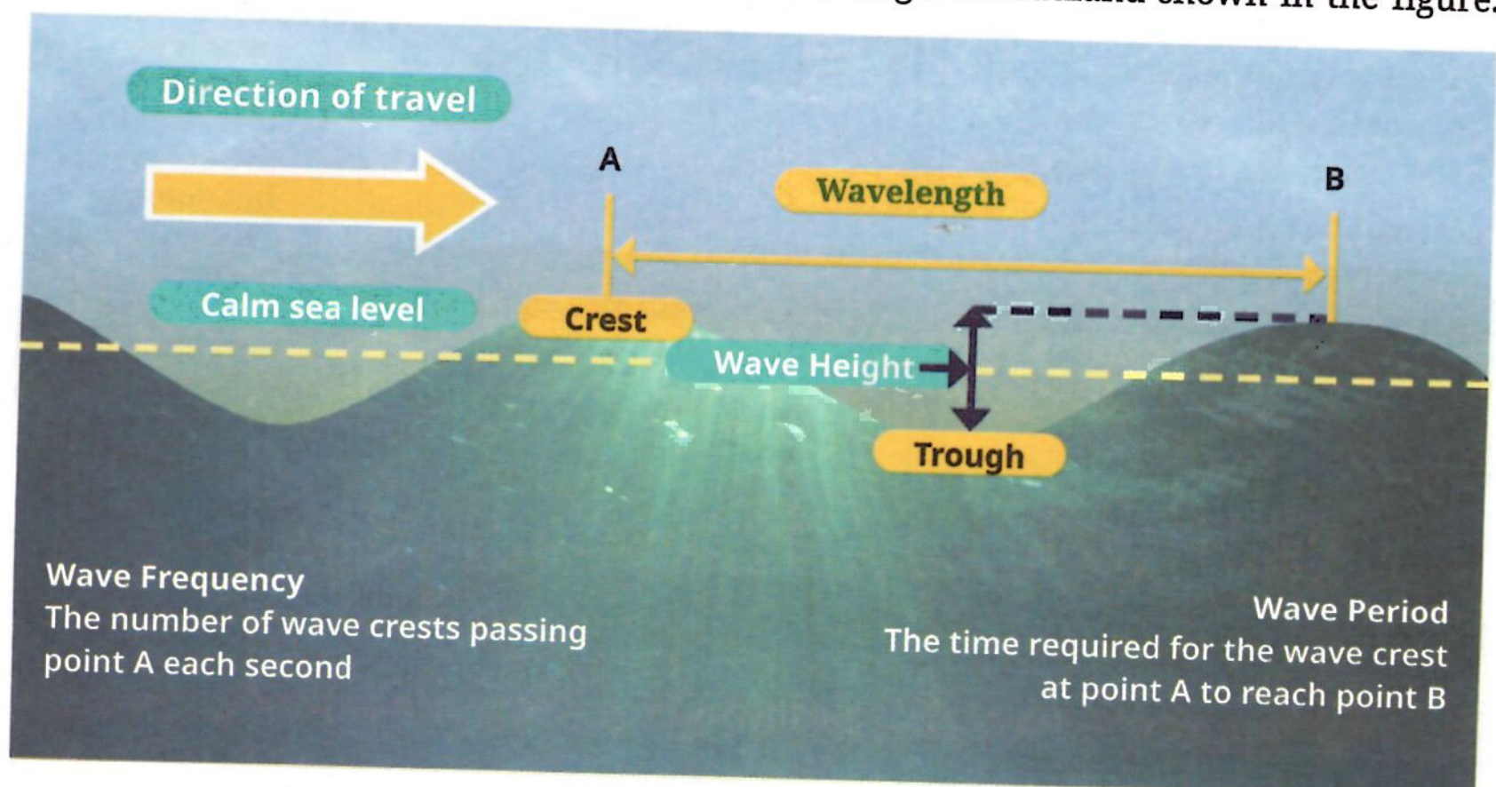
Fig. 1.3. Anatomy of waves
